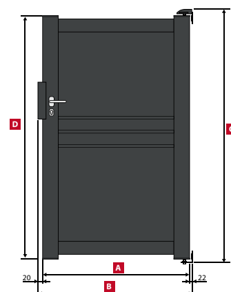
HOUSTON Portillon / Side gate / Gartentür
