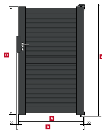
DENIA Portillon / Side gate / Gartentür
