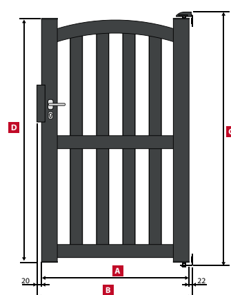
CORAIL Portillon / Side gate / Gartentür
