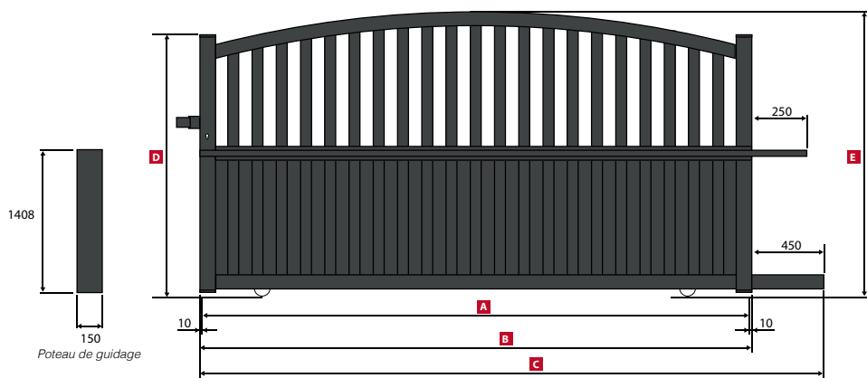
PHILIPPINES Portail Coulissant / Sliding gate / Schiebetor
