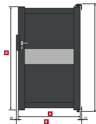
MEMPHIS Portillon / Side gate / Gartentür
