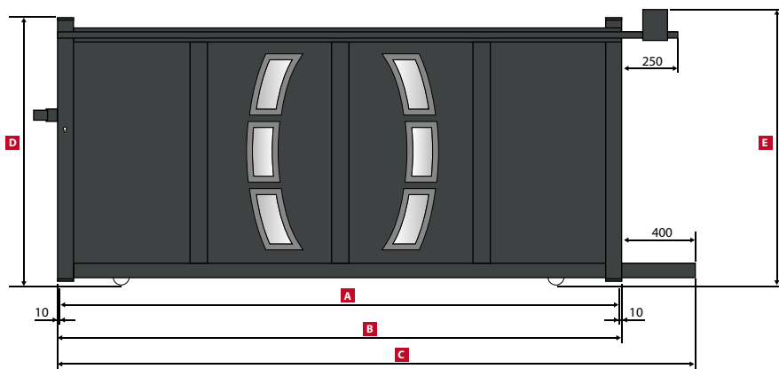
SEATTLE Portail Coulissant / Sliding gate / Schiebetor
