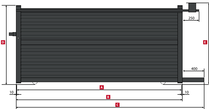
DENIA Portail Coulissant / Sliding gate / Schiebetor
