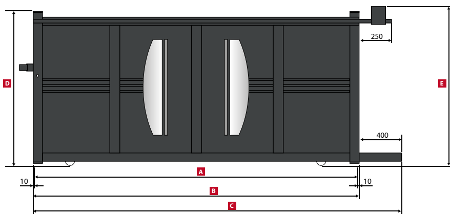
HOUSTON Portail Coulissant / Sliding gate / Schiebetor
