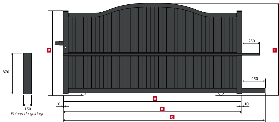
MARMARA Portail Coulissant / Sliding gate / Schiebetor
