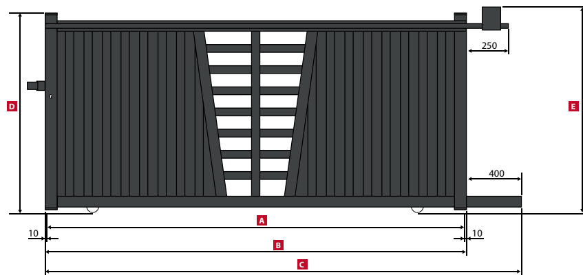
LICOLIN Portail Coulissant / Sliding gate / Schiebetor
