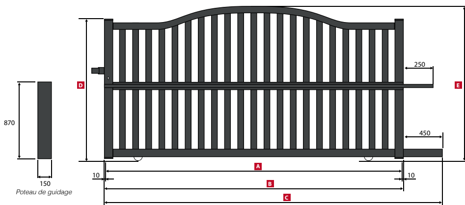
BERING Portail Coulissant / Sliding gate / Schiebetor
