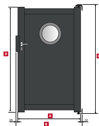
CHICAGO Portillon / Side gate / Gartentür
