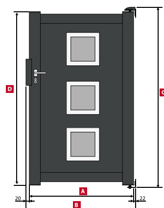
DAYTON Portillon / Side gate / Gartentür
