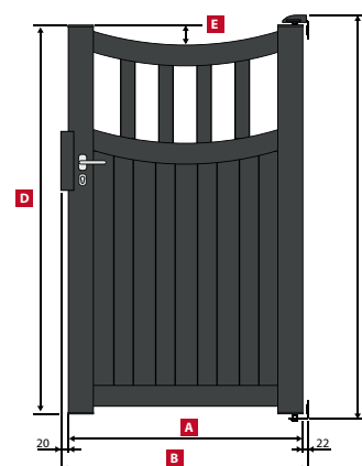
BENGAL Portillon / Side gate / Gartentür
