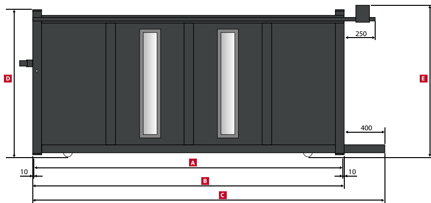
DALLAS Portail Coulissant / Sliding gate / Schiebetor
