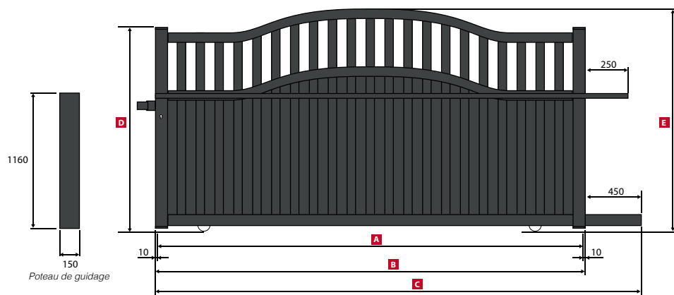
FLORES Portail Coulissant / Sliding gate / Schiebetor
