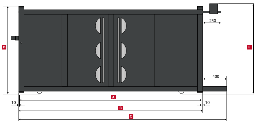
TRENTON Portail Coulissant / Sliding gate / Schiebetor
