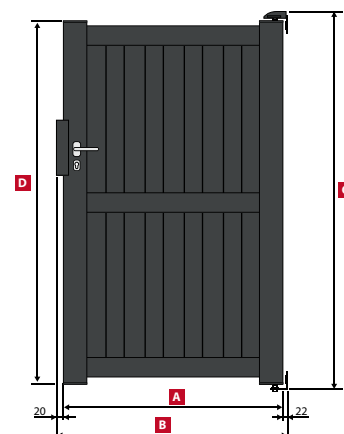
MELVILLE Portillon / Side gate / Gartentür
